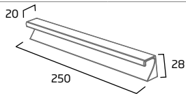
250mm Recessed Handle
