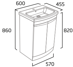
600mm Freestanding Wash Unit
