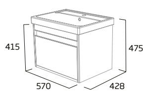
600mm Wall Mounted Wash Unit
