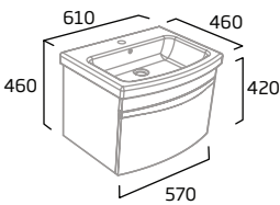
600mm Wall Mounted Wash Unit
