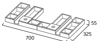
800mm Storage Pack 6
