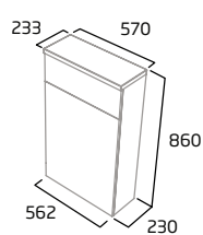
Back to Wall WC Unit
