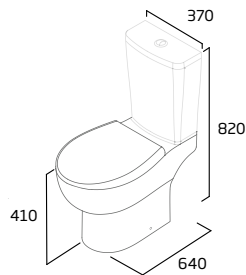
Standard Height Close Coupled WC
