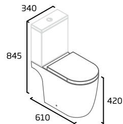
Standard Height Close Coupled WC
