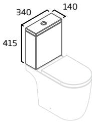
Standard WC Cistern with Contactless Flush
