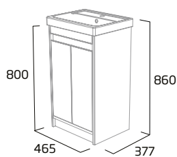
500mm Freestanding Wash Unit
