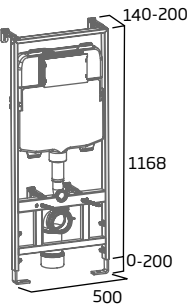
1.17m Wall Hung WC Frame
