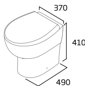
Back To Wall WC
