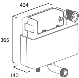
Concealed Dual Flush Cistern (Bottom Entry Inlet)
