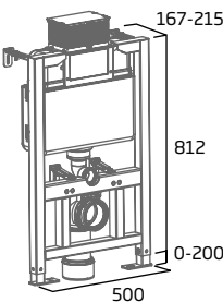
0.82m Wall Hung WC Frame
