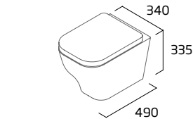
Wall Hung WC
