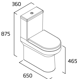
Rimless Comfort Height Fully Enclosed WC
