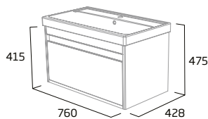
800mm Wall Mounted Wash Unit
