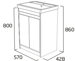
600mm Freestanding Wash Unit
