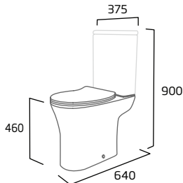
Comfort Height Close Coupled WC
