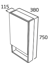
400mm Single Door Cabinet
