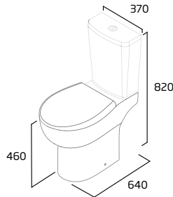
Comfort Height Close Coupled WC
