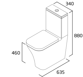
Comfort Height Fully Enclosed Close Coupled WC
