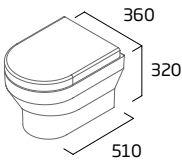
Rimless Wall Hung WC
