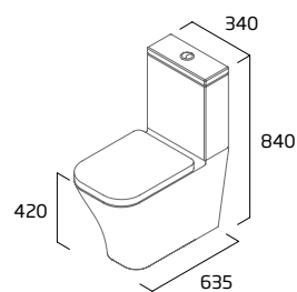
Fully Enclosed Close Coupled WC
