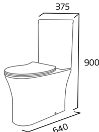
Comfort Height Fully Enclosed Close Coupled WC
