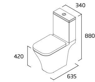
Comfort Height Standard Close Coupled WC
