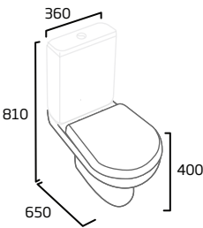
Rimless Standard Close Coupled WC
