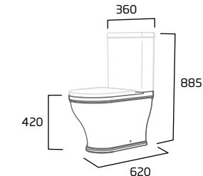
Fully Enclosed Close Coupled WC
