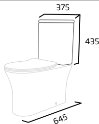
Standard WC Cistern (Fits Fully Enclosed and Open Back WC)
